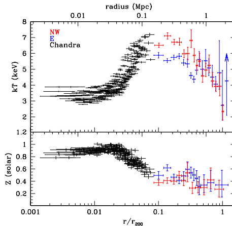
Figure 19: The observed, projected temperature ( kT ) and metallicity ( Z ) profiles in the Perseus Cluster, the nearest, massive galaxy cluster and brightest, extended extragalactic X-ray source. Suzaku results for the northwestern (NW) arm of the cluster are shown in red; and for the eastern (E) arm (approximately aligned with the major axis) in blue (Simionescu et al. 2011). Chandra measurements of the inner regions (Sanders & Fabian 2007) are shown in black.
