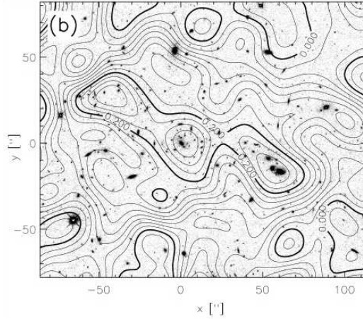
Fig. 23. Mass reconstruction (contours) of the inner part of the high-redshift ( z_d = 0.83 ) cluster MS1054-03, based on a mosaic of six pointings obtained with the WFPC2@HST (from Hoekstra et al. 140). The splitting of the cluster core into three subcomponents, also previously seen from ground-based images by Clowe et al. (2000), shows that this cluster is not yet relaxed
